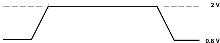
Figure 13. TTL-Level Inputs
