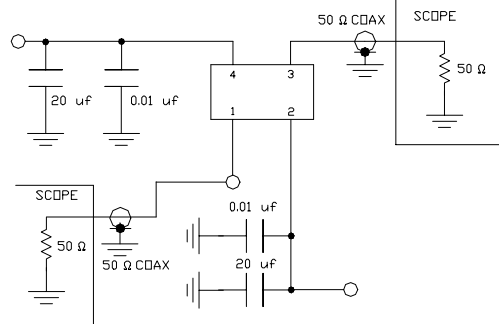
TEST CIRCUIT
