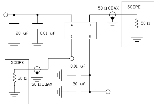
TEST CIRCUIT
