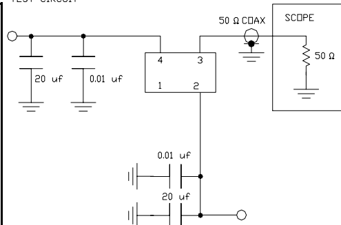
TEST CIRCUIT
