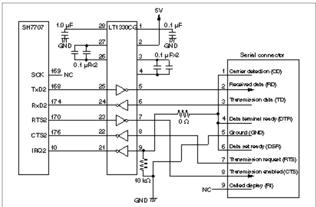
Figure 4.29 SCIF Block Diagram
