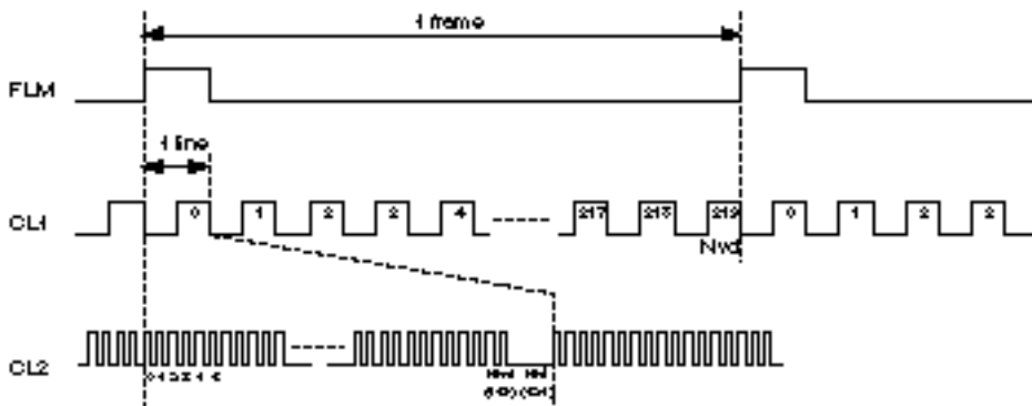
Figure 4.6 Timing Chart
