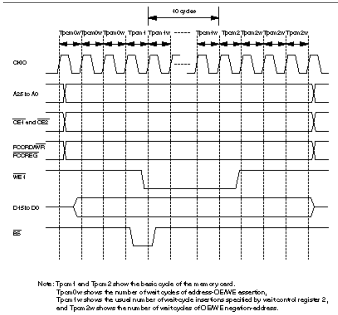
Figure 4.13 Memory Card (4)
