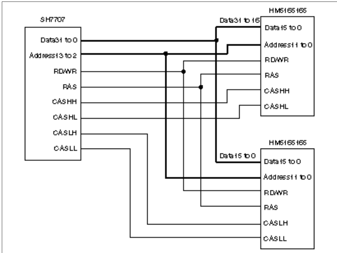
Figure 4.1 DRAM Connection
