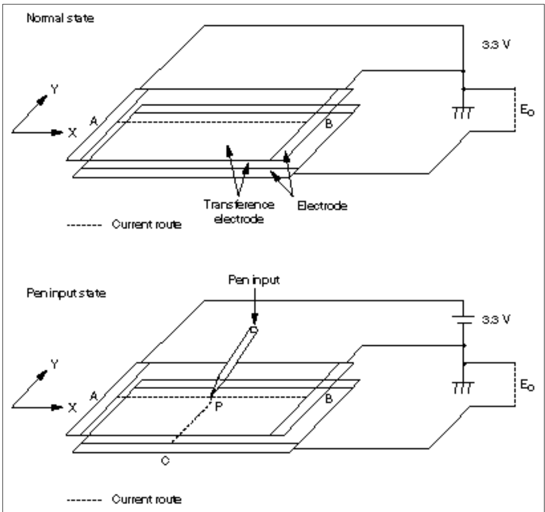
Figure 4.23 Mechanism of a Touch Panel
