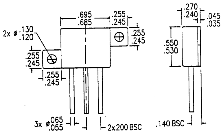
TO-259 (P)
