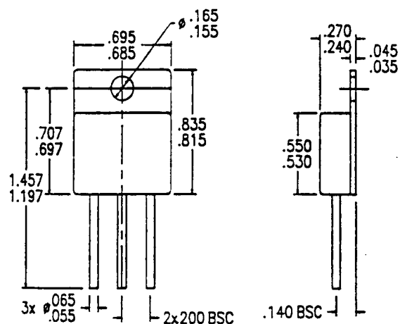
TO-258 (N)
