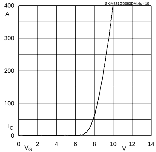
Fig. 10 Typ. transfer characteristic, t_p = 80 \mu s ; V_{CE} = 20 V
