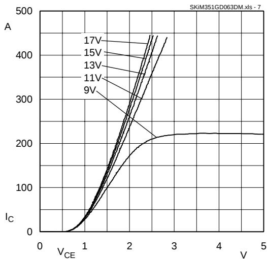
Fig. 7 Typ. output characteristic, t_p = 80 \mu s ; 25 °C
