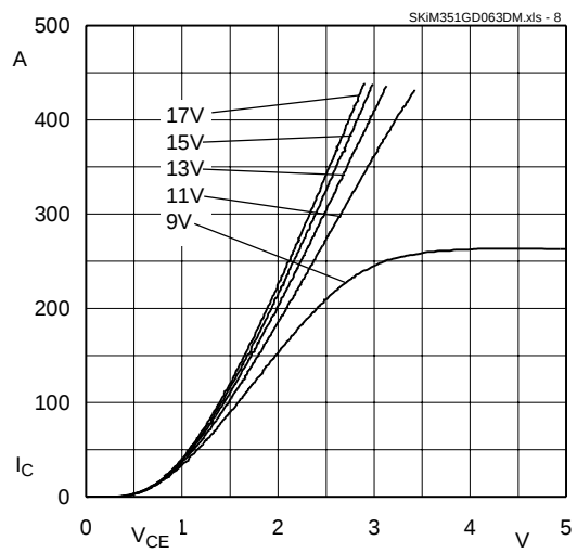
Fig. 8 Typ. output characteristic, t_p = 80 \mu s ; 125 °C
