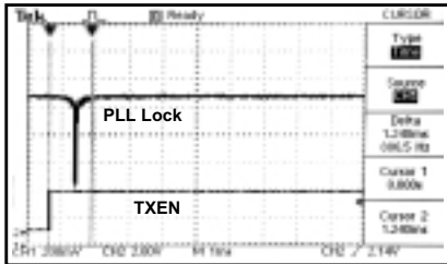
Figure 3: Transmitter Enabled to PLL Lock
