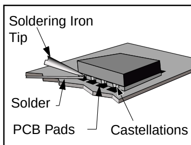
Figure 6: Soldering Technique
