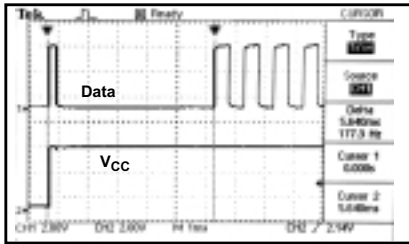
Figure 1: Power-on to valid RX data
