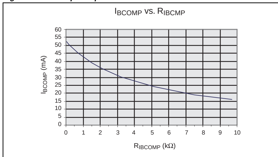
Figure 9. APC Loop Compensation Bias Current vs. IBCMP Resistor Value
