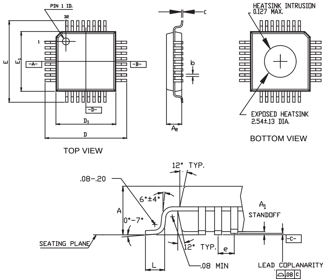
Figure 3. 32 TQPF Package
