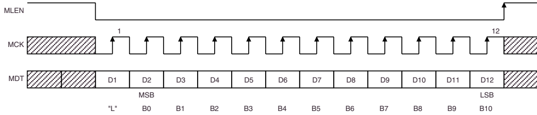
Figure 3. Attenuation data format (microcontroller interface)
