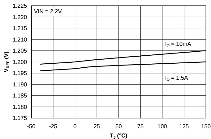
Reference Voltage vs. Junction
