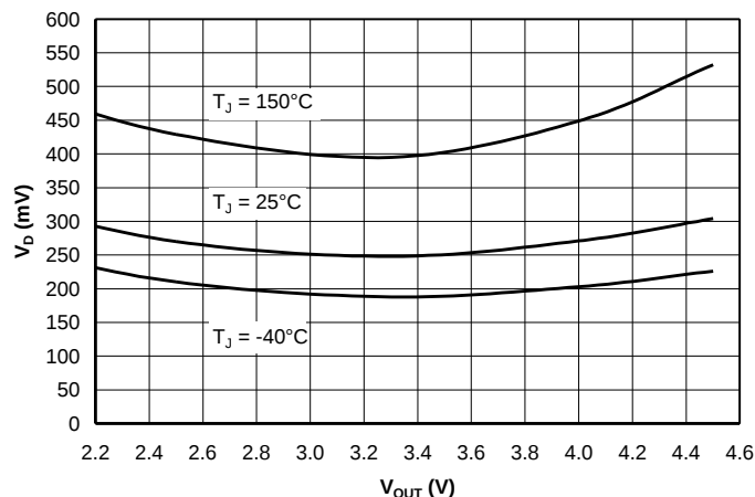
Dropout Voltage ( I_{OUT} = 0.5A ) vs. Output
