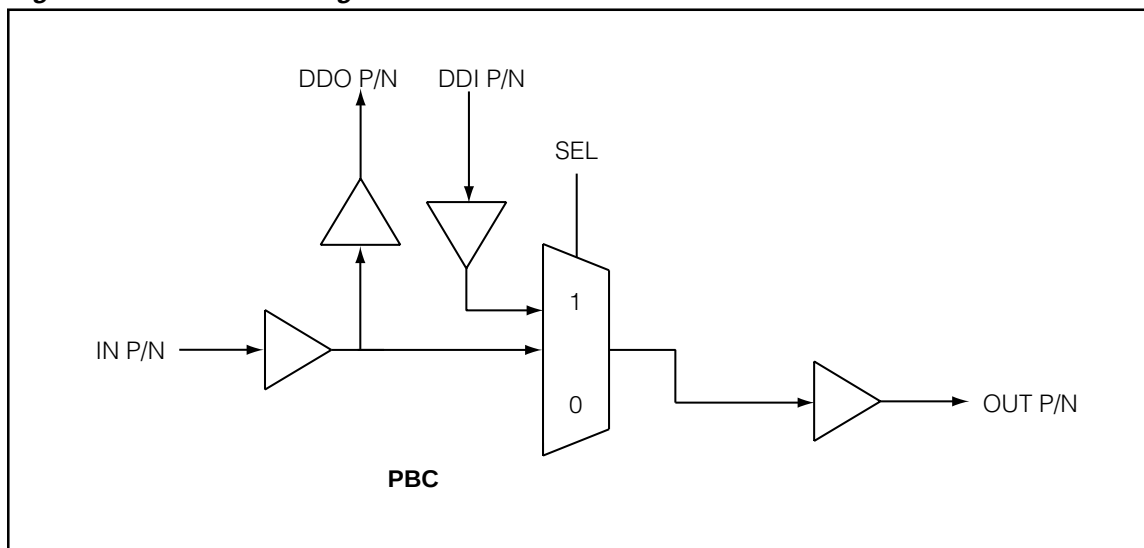
Figure 1. S2091 Block Diagram
