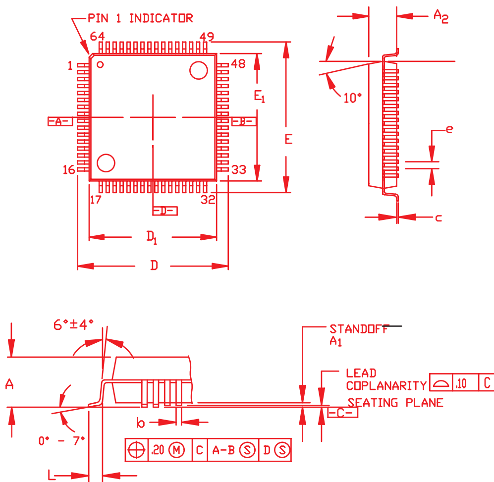
Figure 5. 14mm x 14mm 64 PQFP Package
