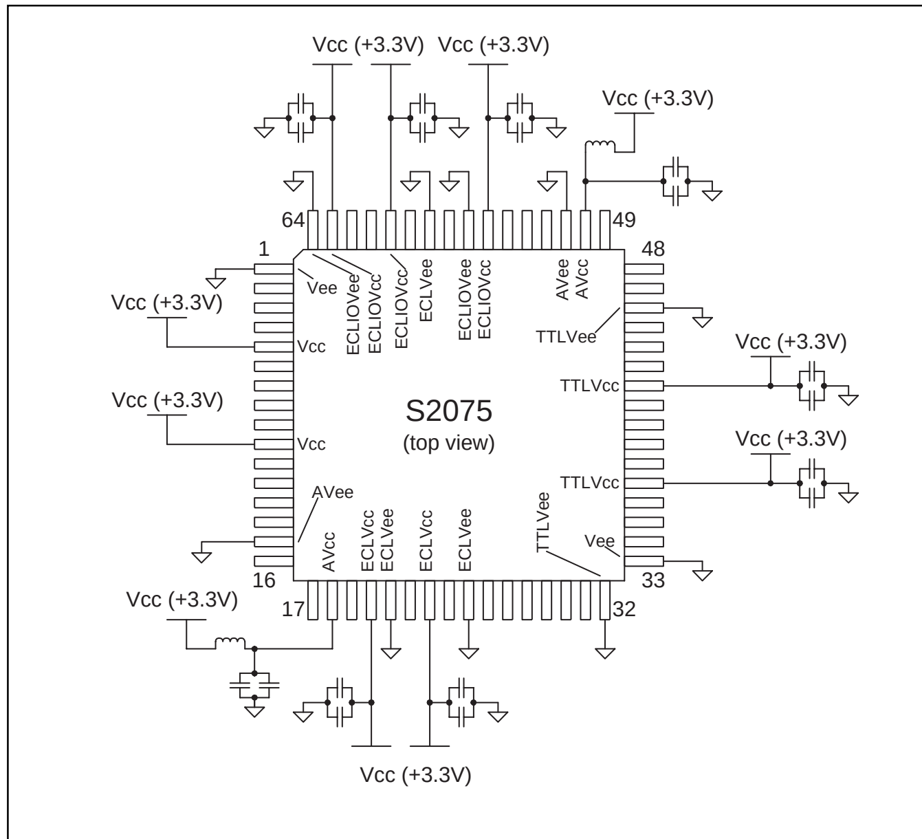
Figure 7. Power and Ground Connection Diagram
