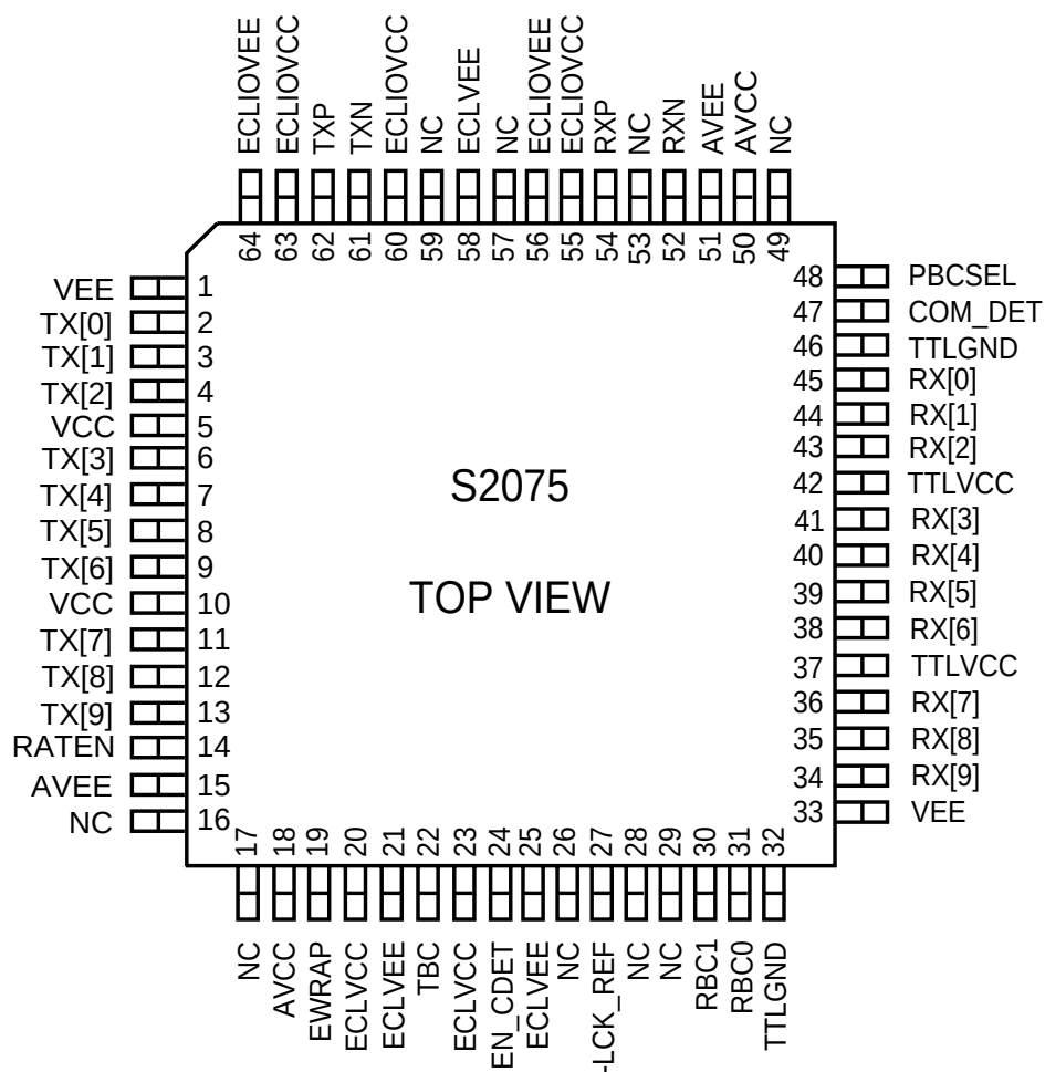
Figure 4. S2075 Pinout
