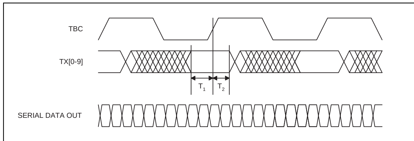
Figure 8. Transmitter Timing
