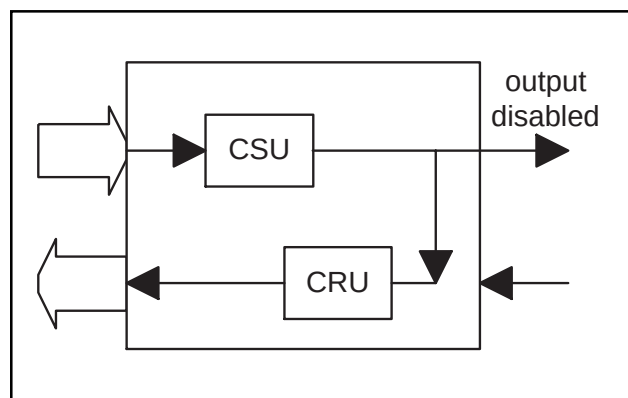
Figure 11. Loopback Operation
