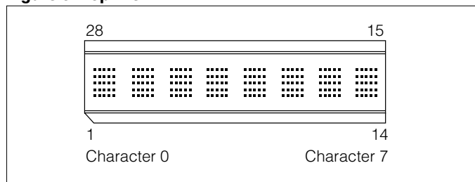
Figure 3. Top View
