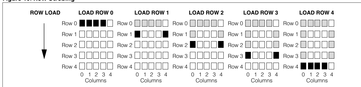
Figure 10. Row Strobing
