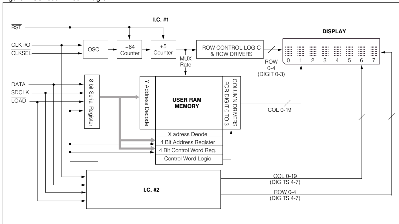
Figure 7. SCD558X Block Diagram
