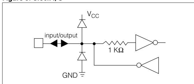
Figure 5. Clock I/O
