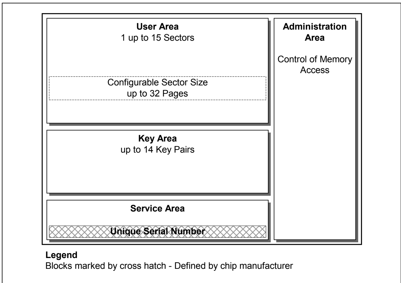
Figure 3 Memory principle of SLE 55R02
