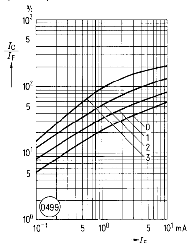
Figure 7. Current Transfer Ratio versus Diode Current ( T_A=75^\circ\text{C} , V_{CE}=5.0\text{ V} )
