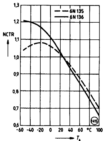
Figure 16. Current Transfer Ratio (normalized) vs. Ambient Temp.
