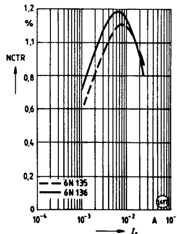
Figure 13. Current Transfer Ratio (normalized) vs. Forward Current I_F=16\text{ mA} , V_O=0.4\text{ V} , V_{CC}=5.0\text{ V} , T_A=25^\circ\text{C}
