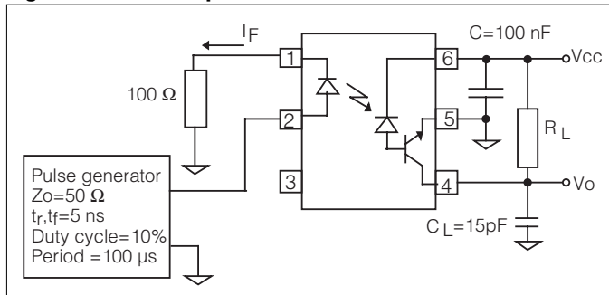
Figure 1. Test Set-up
