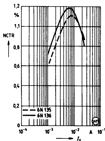
Figure 19. Current Transfer Ratio (normalized) vs. Forward Current
