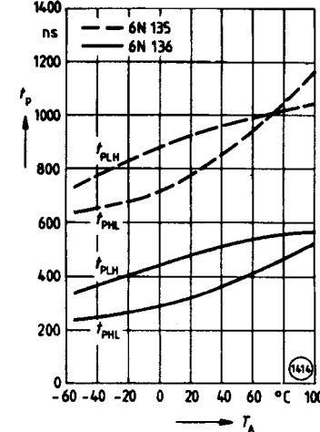
Figure 12. Delay Times vs. Ambient Temperature I_F=16\text{ mA} , V_{CC}=5.0\text{ V} , R_L=4.1\text{ k}\Omega , SFH6136: R_L=1.9\text{ k}\Omega
