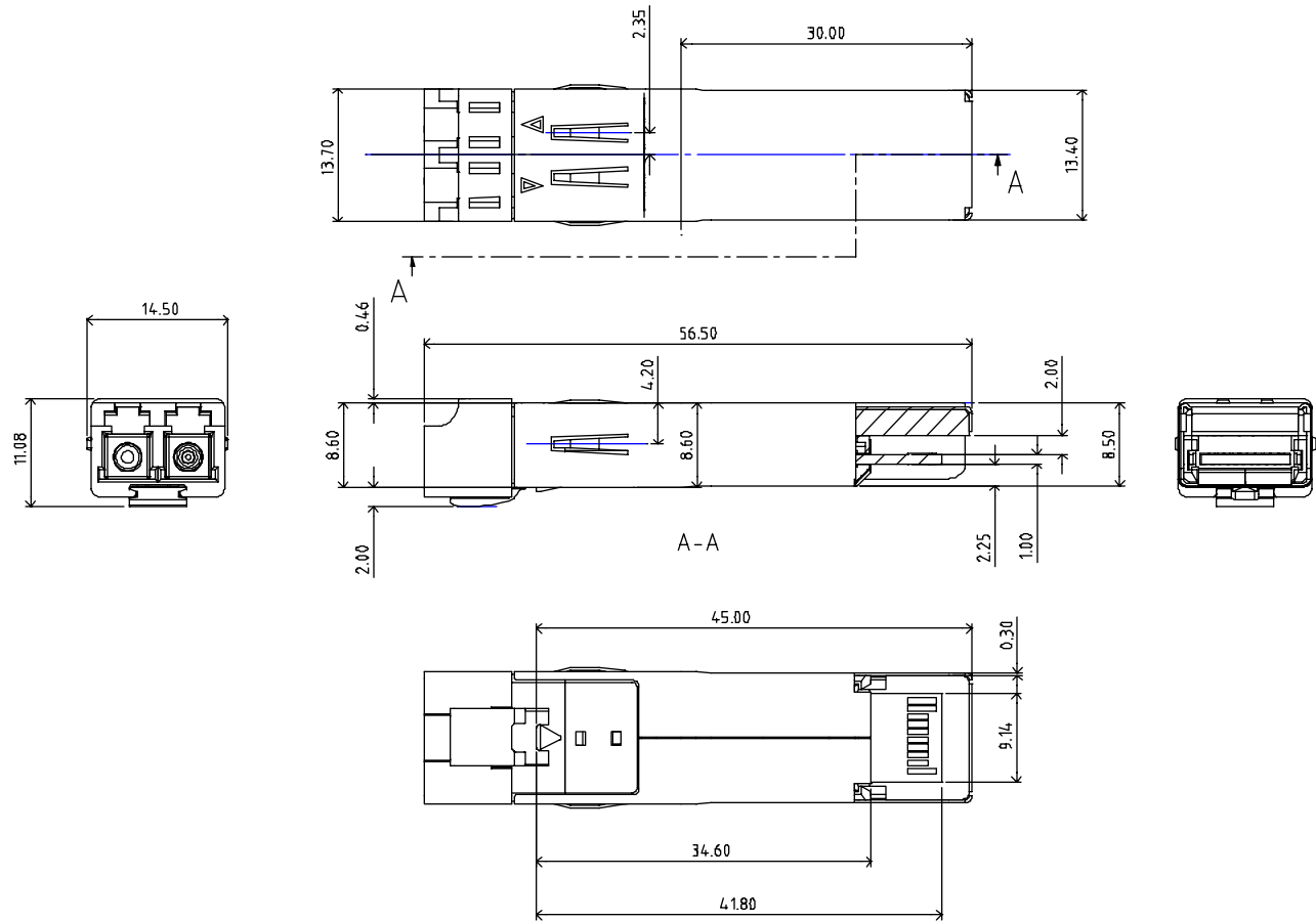
Figure 2. Outline Dimensions
