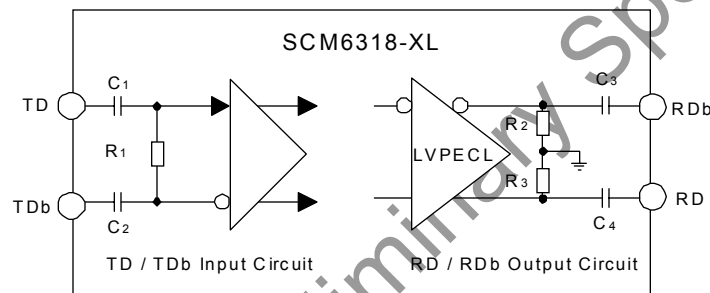
Figure 15. Data Input / Output Circuit
