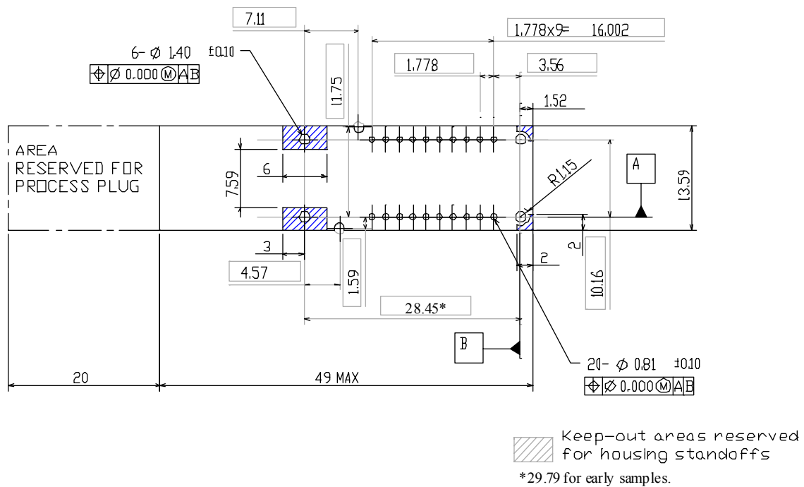
Figure 7. Recommended Footprint
