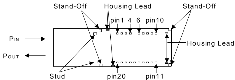
Figure 9. Pin Location ( Bottom View )
