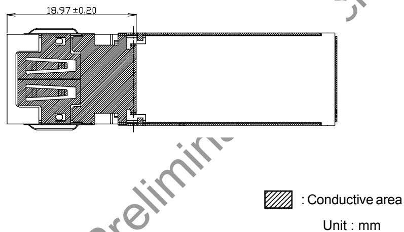
Figure 6. Package Bottom View
