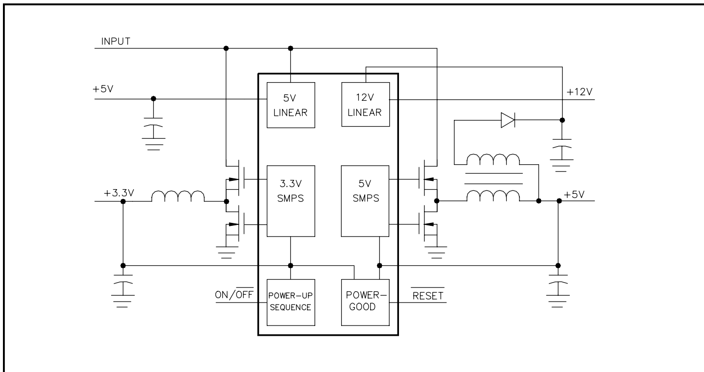
PWM Controller Diagram (Fig. 1)
