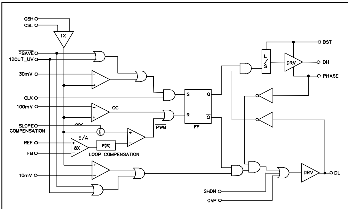
PWM Controller Diagram (Fig. 1)
