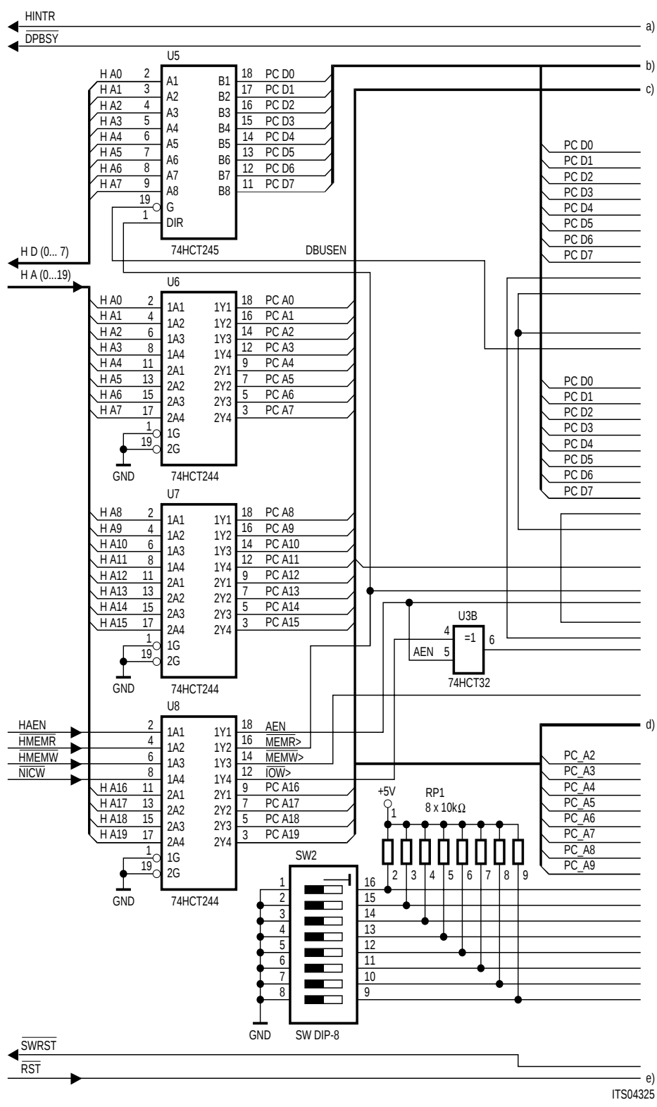
PC-Bus Interface-Logic
