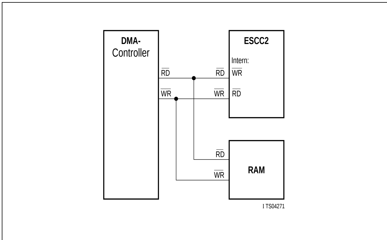
Figure 5 \overline{RD} -/ \overline{WR} -Exchange
