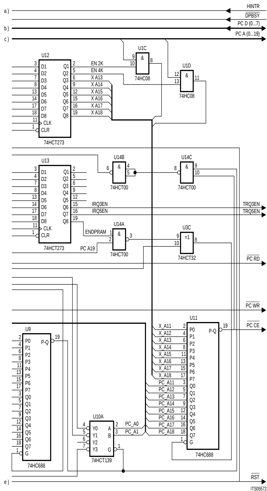
PC-Bus Interface-Logic (cont'd)
