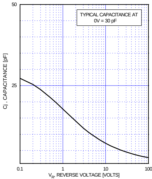
Fig.3 Typical Capacitance
