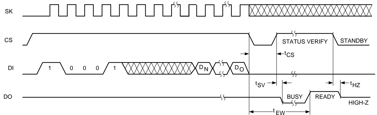
Figure 7. WRAL Instruction Timing
