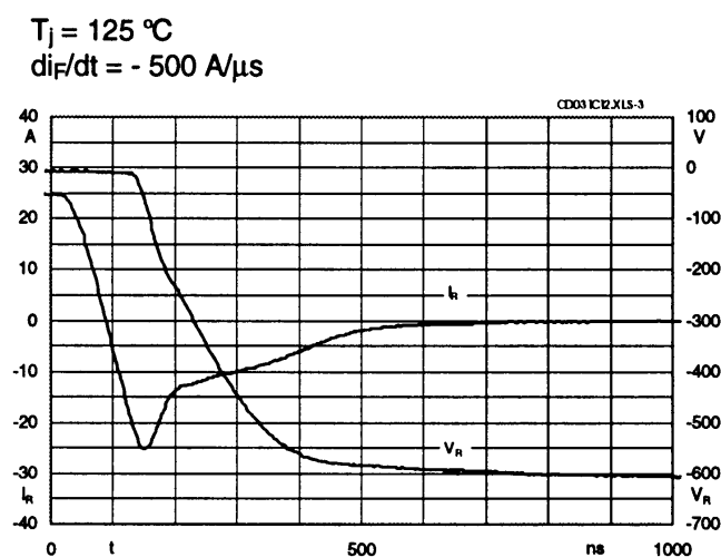
Fig. 3 Typ. diode reverse recovery behaviour i = f (t)
