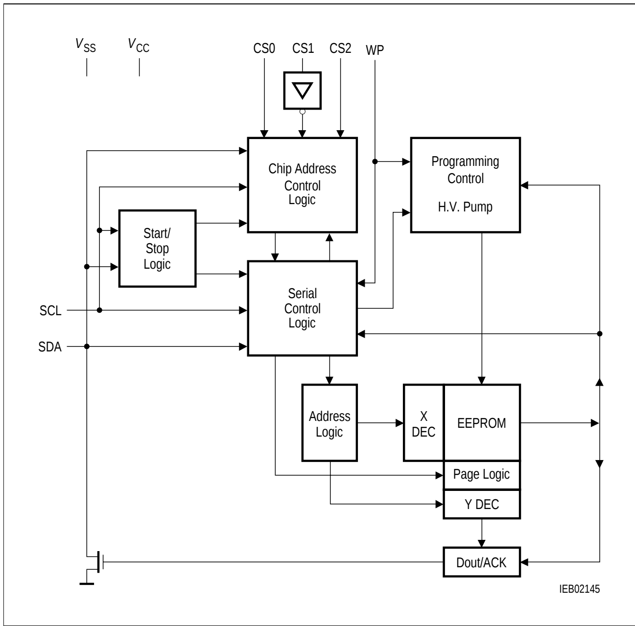
Figure 2 Block Diagram
