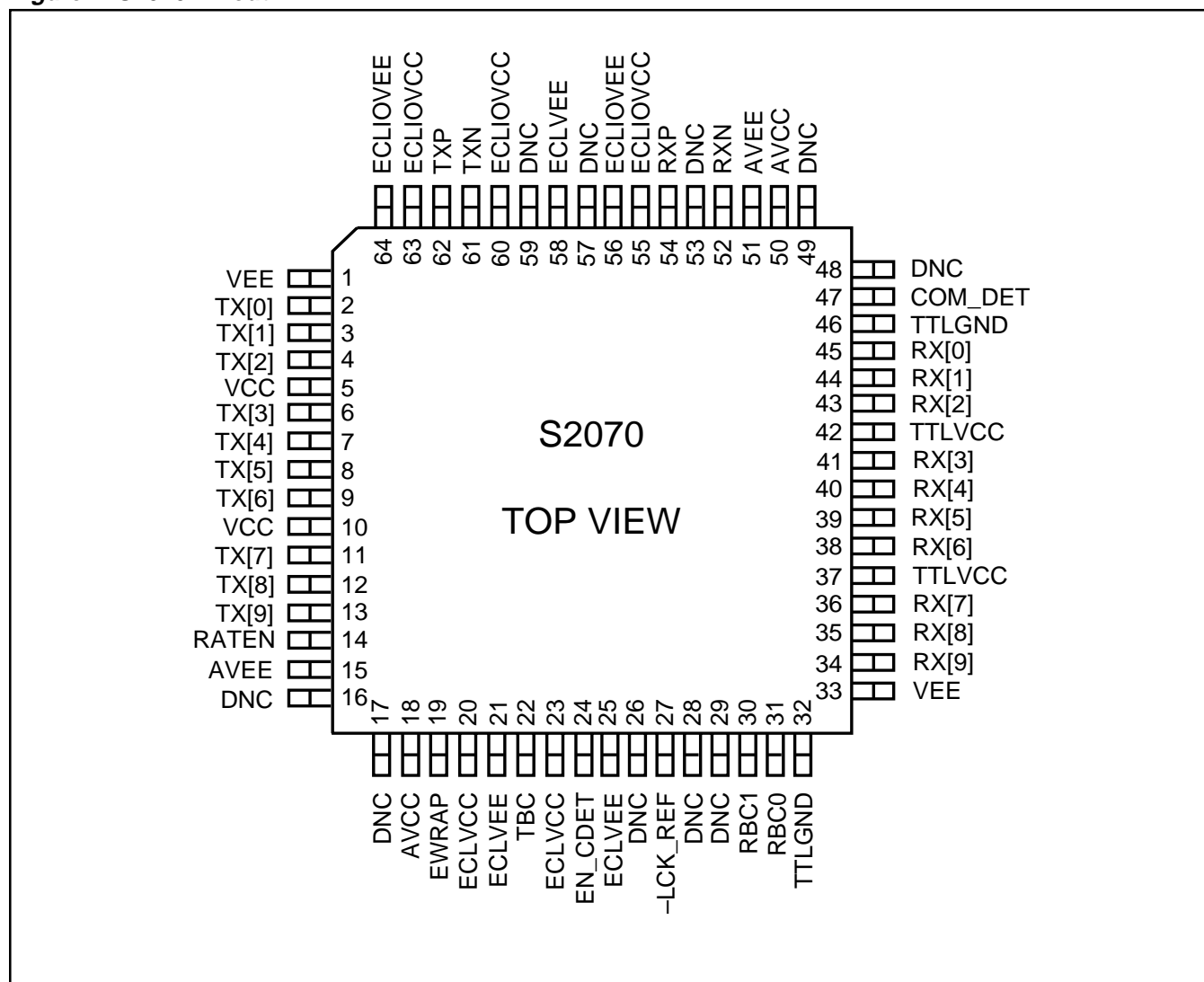
Figure 4. S2070 Pinout
