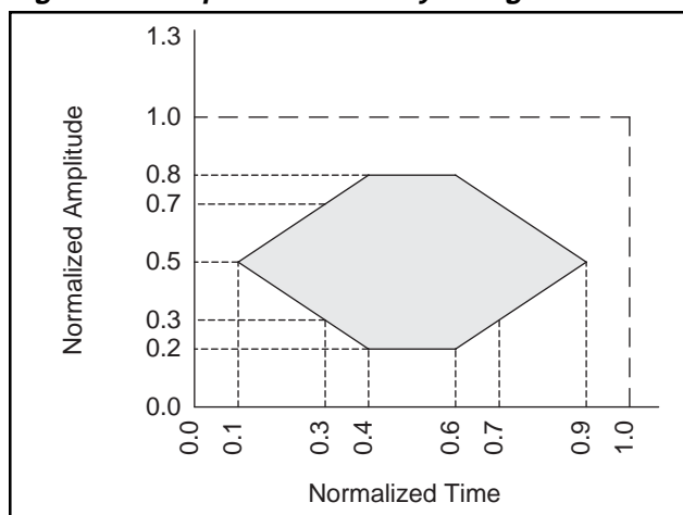
Figure 16. Acquisition Time Eye Diagram
