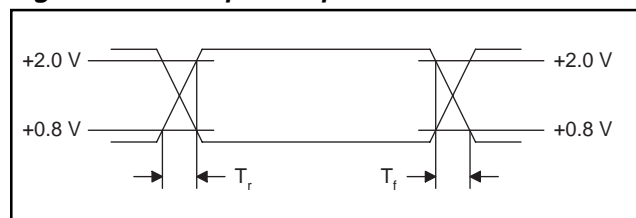
Figure 12. TTL Input/Output Rise and Fall Time
