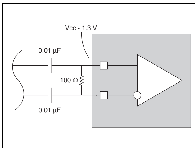
Figure 14. High Speed Differential Inputs
