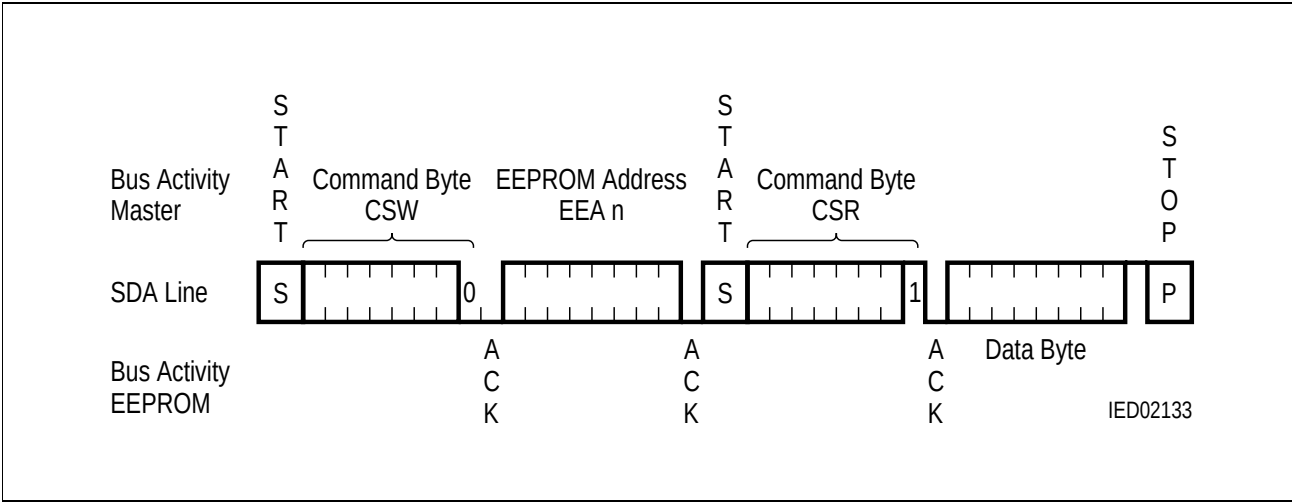
Figure 11 Random Read
