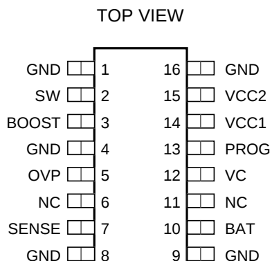
(16 Pin QSOP)
