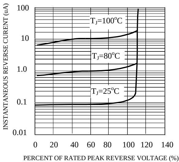
FIG. 3-TYPICAL REVERSE CHARACTERISTICS
