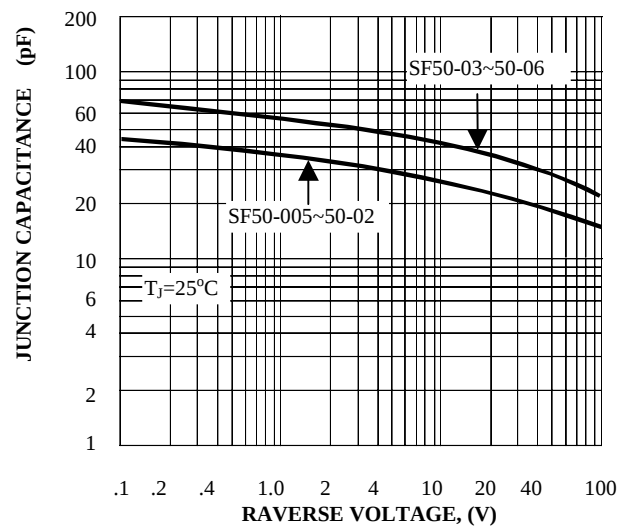
FIG. 6-TYPICAL JUNCTION CAPACITANCE
