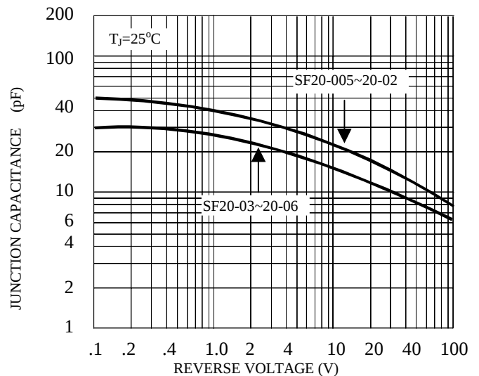
FIG. 6-TYPICAL JUNCTION CAPACITANCE
