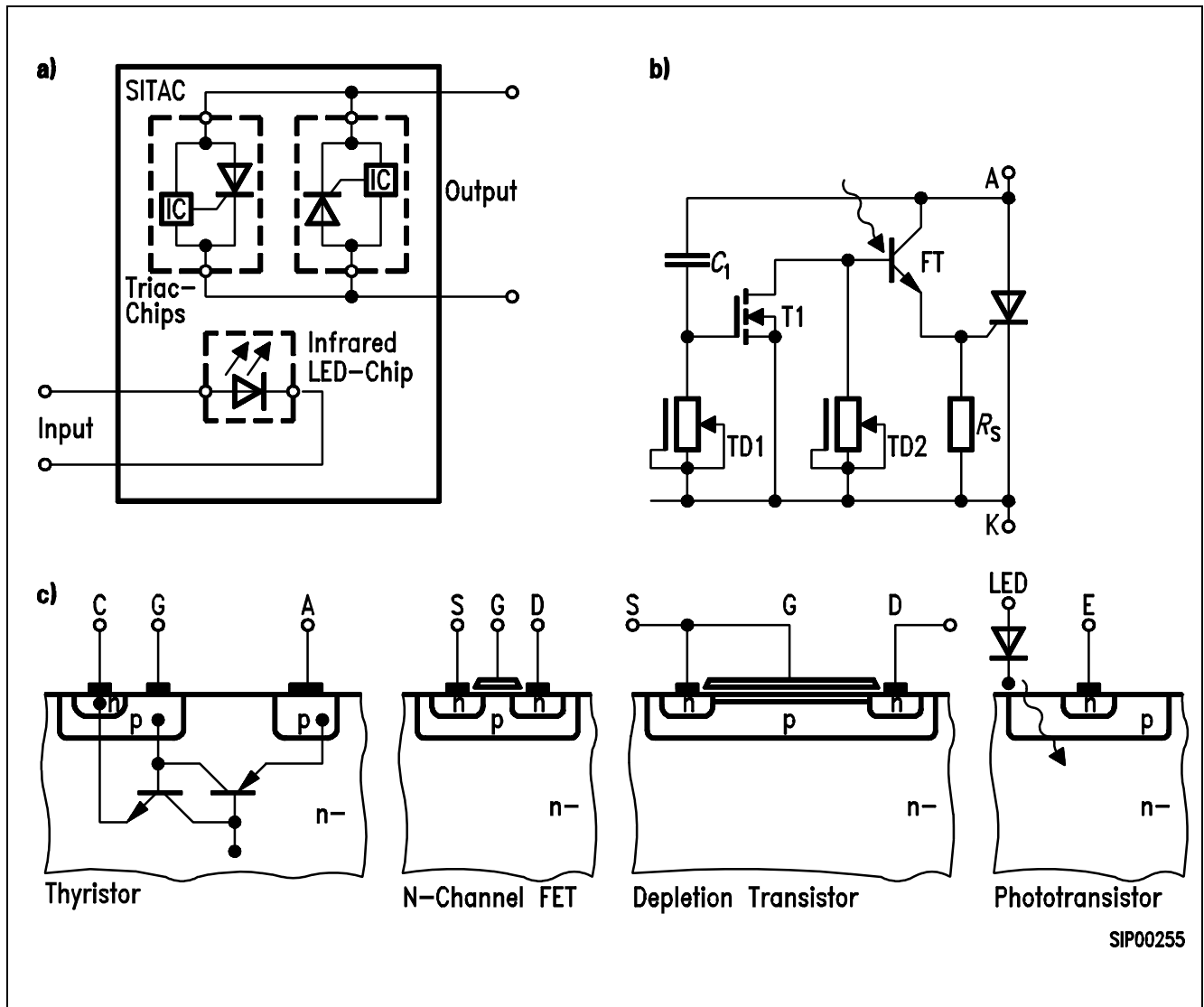
Figure 1 Principle of the SITAC a) Block Diagram of the SITAC Opto-Triac b) Circuit Diagram of a SITAC Branch c) SITAC Semiconductor Branch Elements
