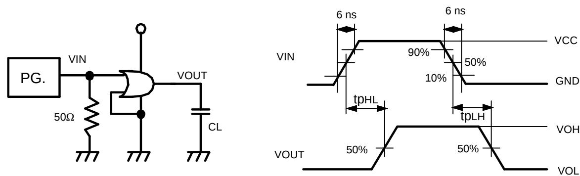
Measurement Circuit
