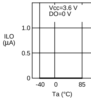
1.11 Output leakage current I_{LO} -- Ambient temperature T_a
