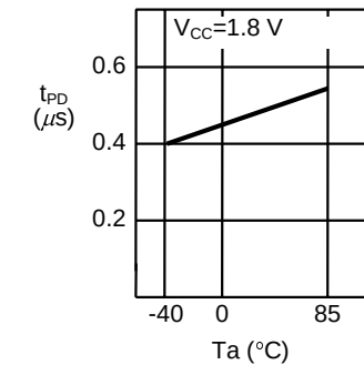
2.7 Data output delay time t PD – Ambient temperature Ta
