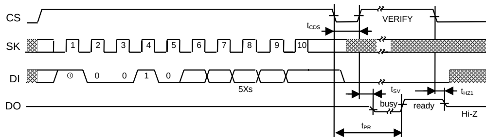
Figure 21 ERAL Timing (S-29231A)
