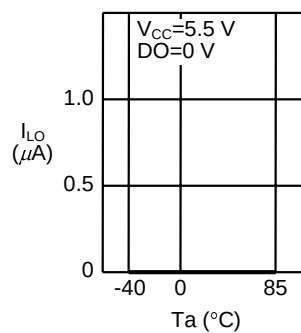
1.14 Output leakage current I_{LO} - Ambient temperature T_a
