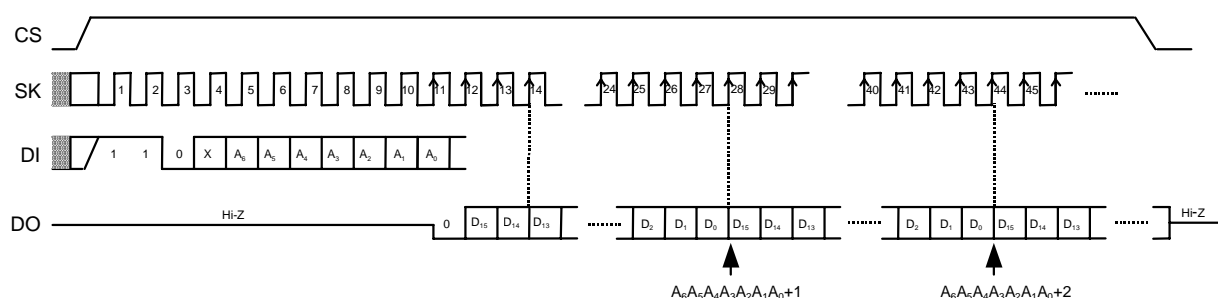
Figure 5 Read Timing (S-29U220A)
