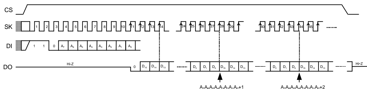
Figure 6 Read Timing (S-29U330A)
