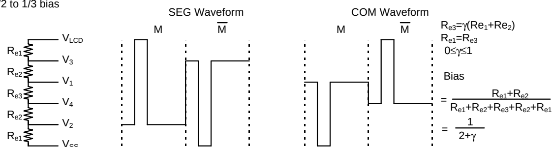
Figure 17 External Bias Resistor vs LCD Drive Waveform
