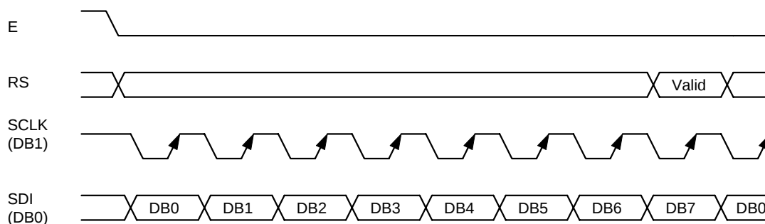
Figure 7 Serial Interface
