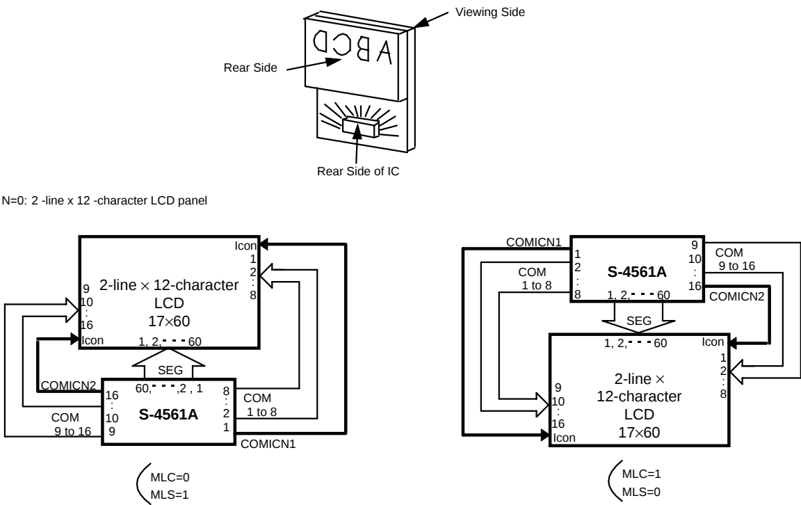
Figure 14: 2-line x 12-character LCD panel
