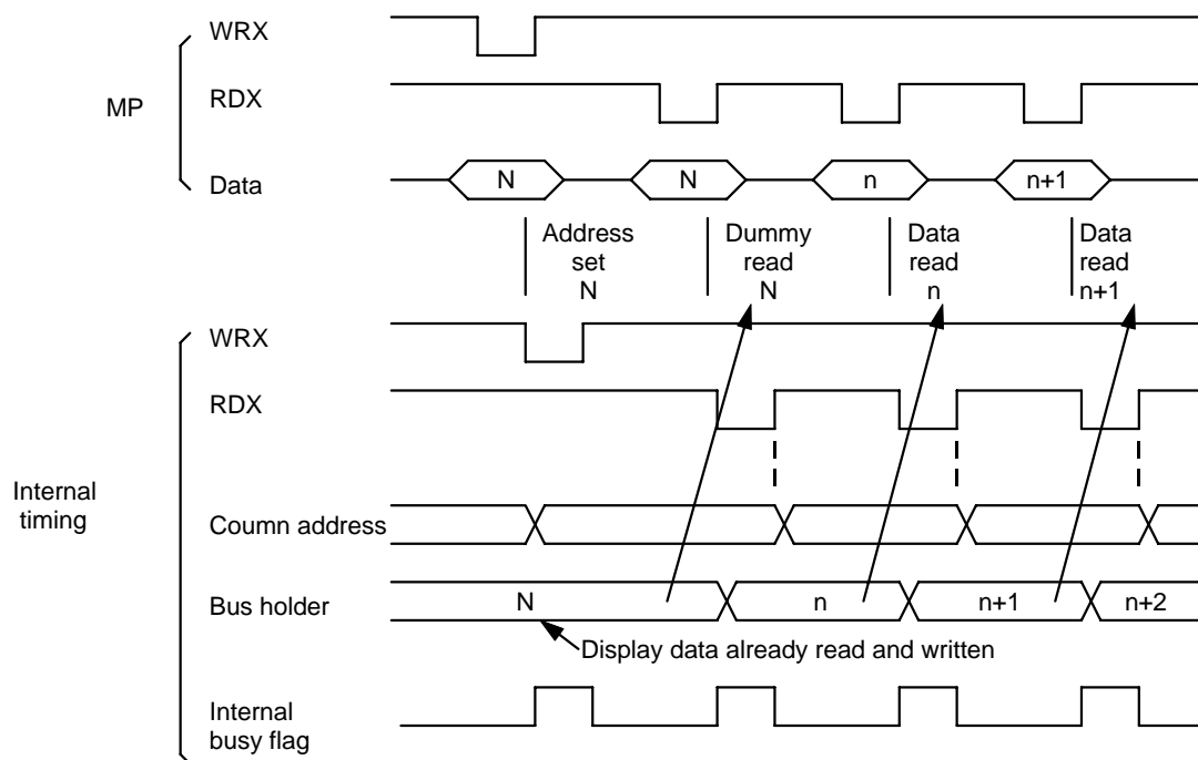
Figure 5 Display data read timing (80 family interface)
