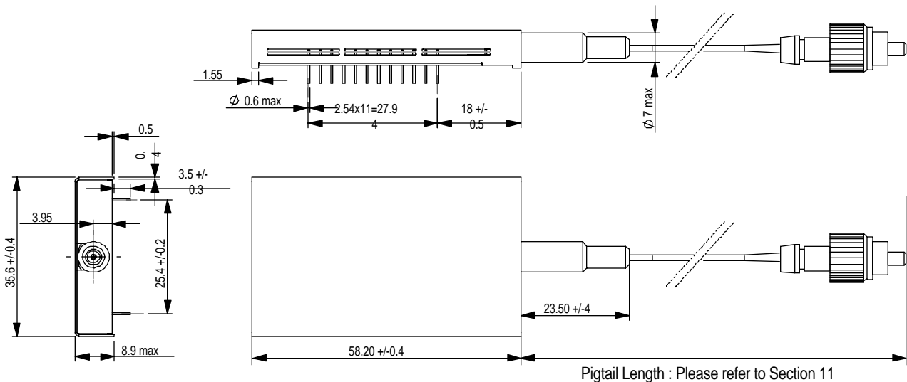
Figure 2 Package Dimension
