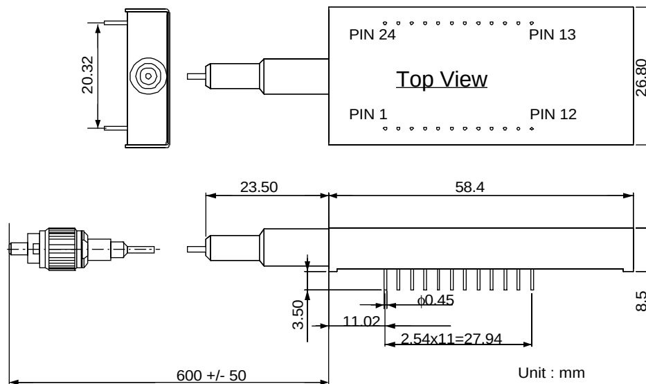
Figure 2. Package Dimension
