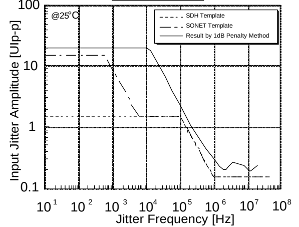
Jitter Tolerance
