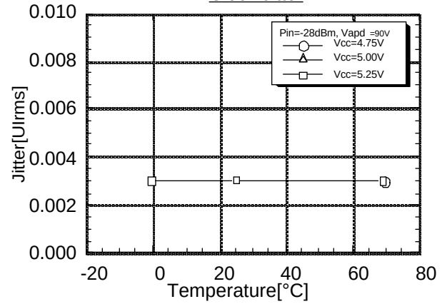
Clock Jitter
