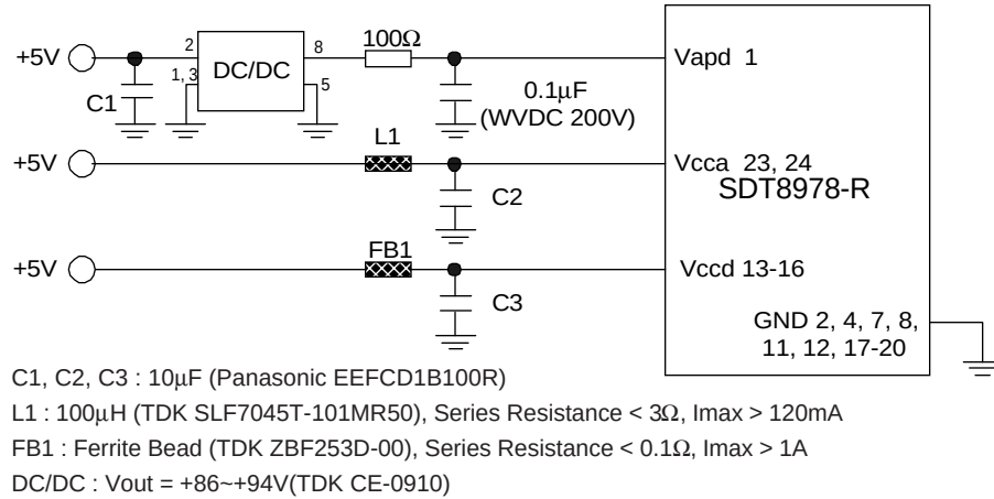
Figure 5 Recommended Power Supply Filtering
