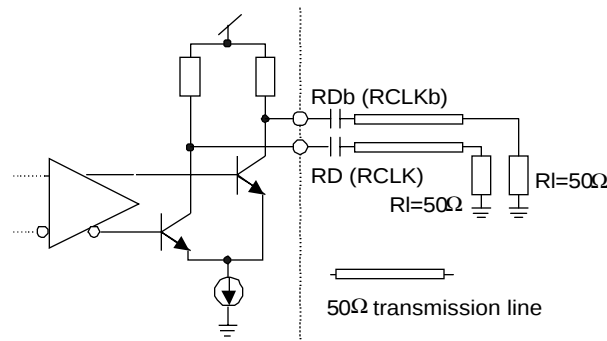
Figure 3 Data and Clock Output Interface (CML Interface)
