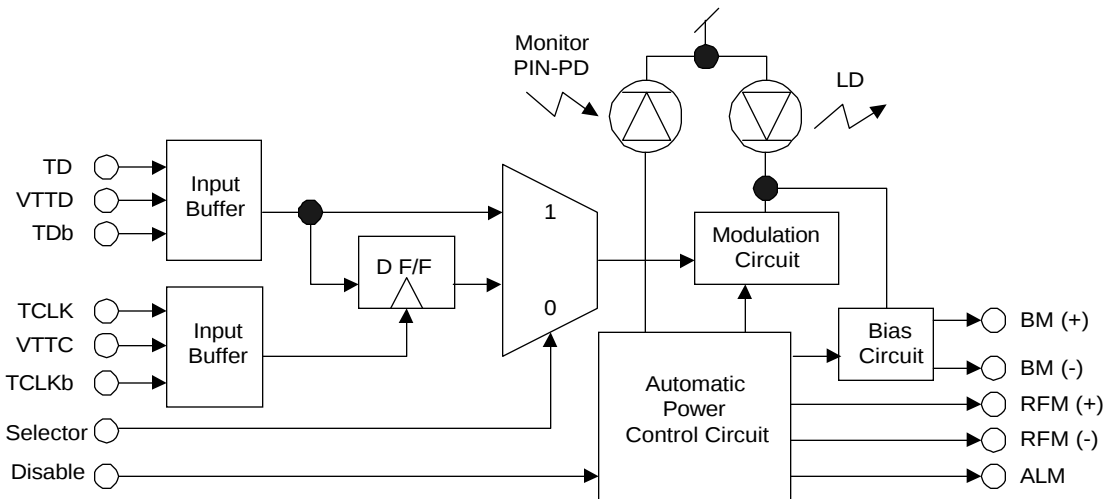
Figure 1 Block Diagram
