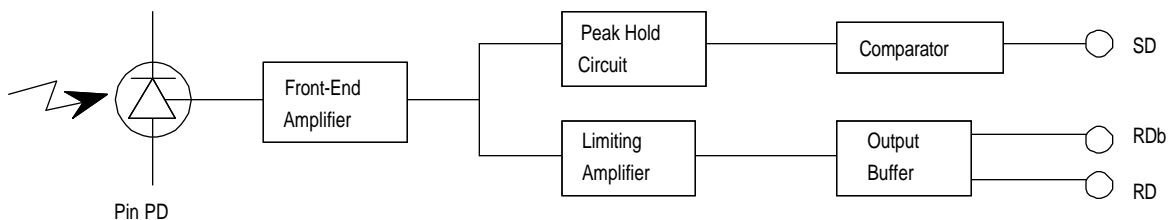
Figure 1-2. Block Diagram(Receiver )
