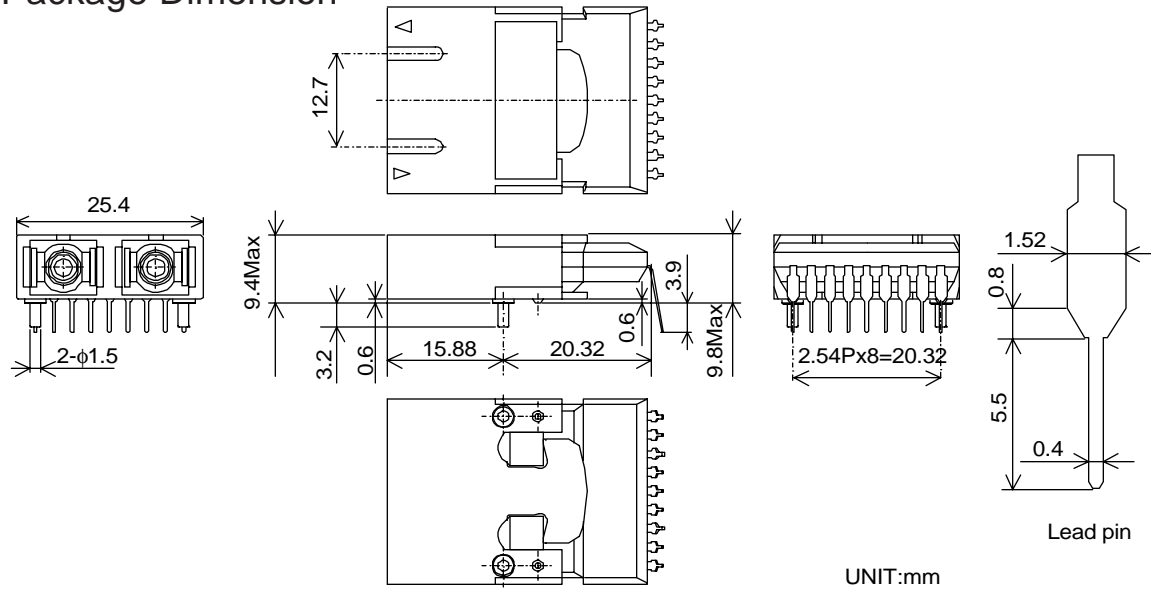
Figure 2. Package Dimension
