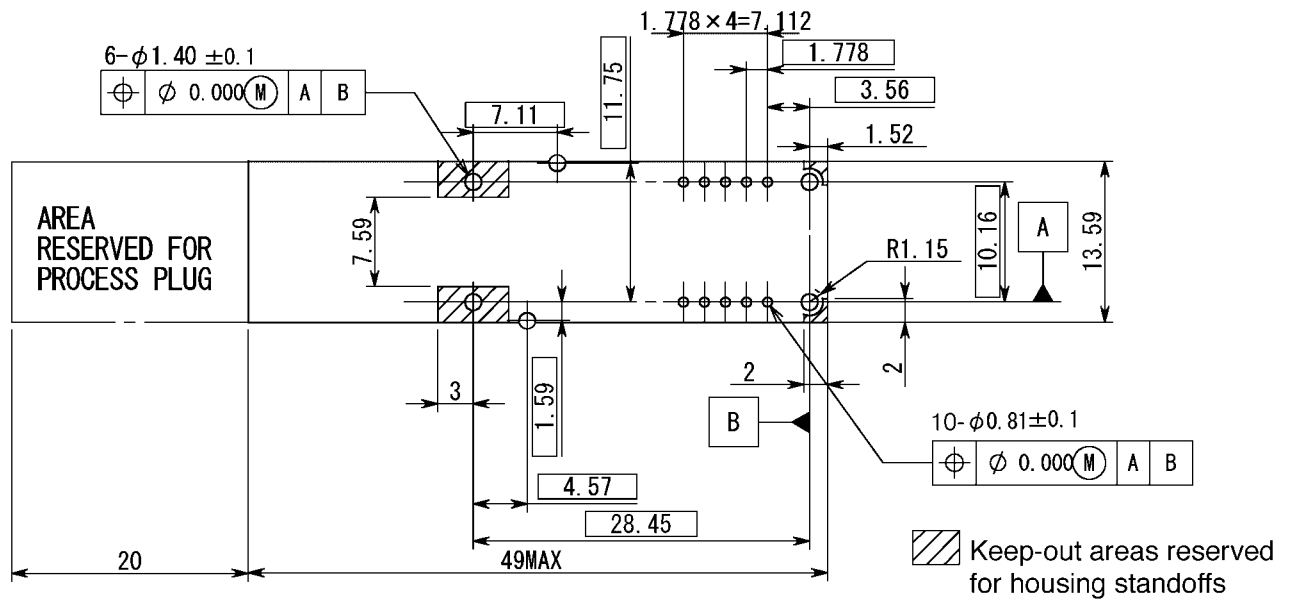
Figure 2-3. Recommended Footprint
