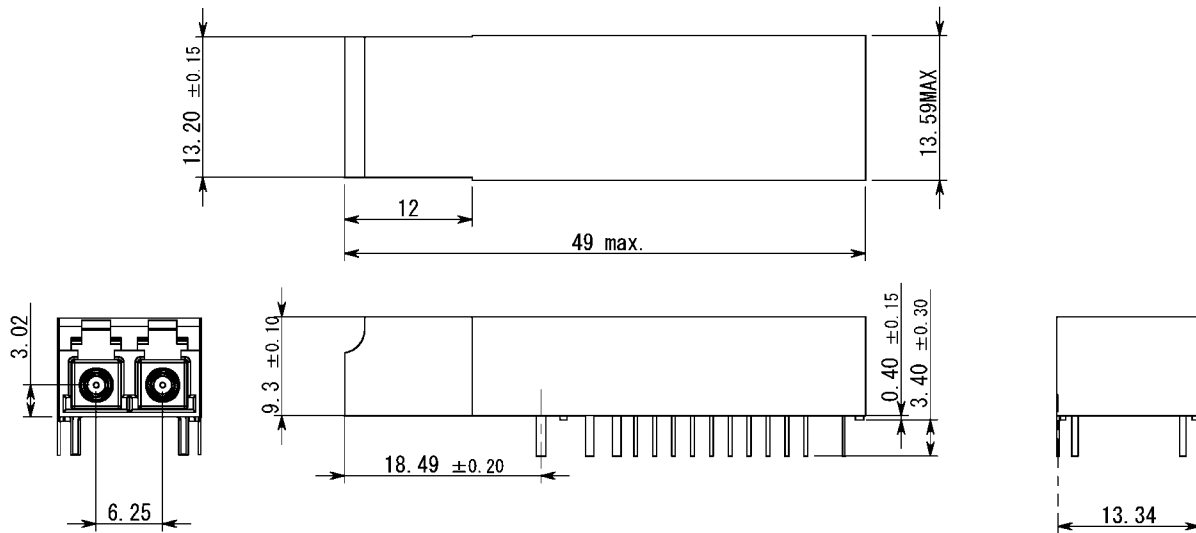
Figure 2-1. Outline Dimensions (SCM6102-GL-Z#)
