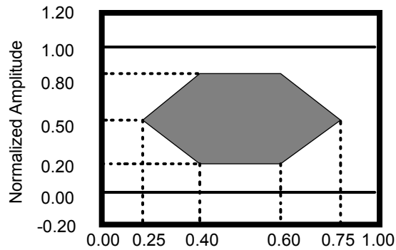
Figure 7. Optical Pulse Mask with Fourth Order
