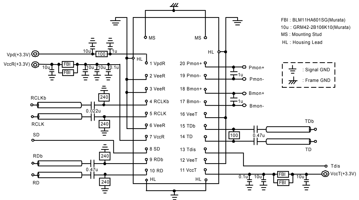
Figure 8. Recommended Interface Circuit
