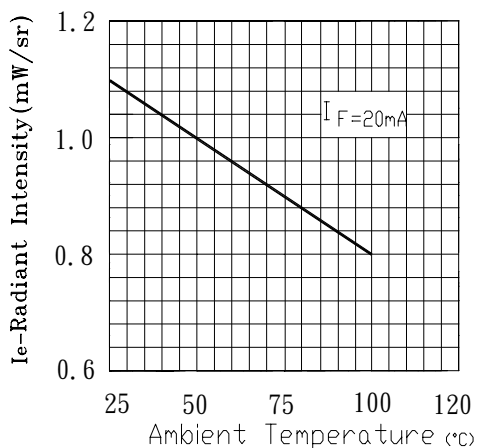
Fig. 7 Relative Intensity vs. Ambient Temperature (°C)
