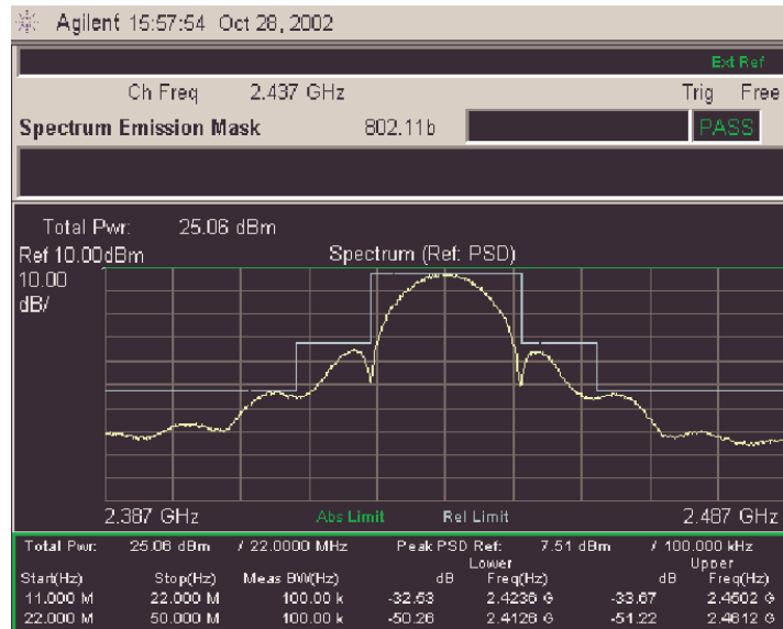
RMPA2453 Spectral Plot Showing Compliance to 802.11b Spectral Mask Requirements @ 25.06 dBm Modulated Output Power 11 Mbps CCK Data 22 MHz BW VC1, VC2 = 3.3V VM12 = 3.3V T=25°C
