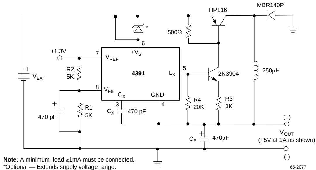
Figure 17. Step-Down High Power Application
