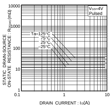
Fig.9 Static Drain-Source On-State Resistance vs. Drain Current (3)
