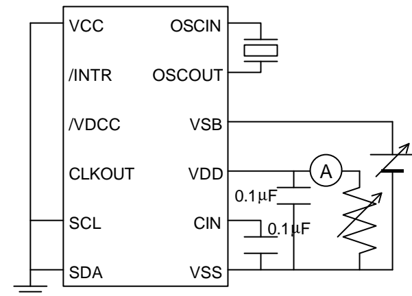
Test circuit
