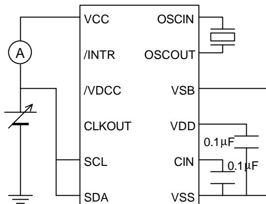
Test circuit
